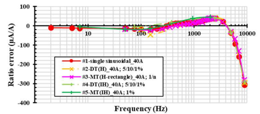
Fig. 3. The frequency response of CT200 for the ratio errors and the ratio errors of CT200 under PQ harmonics / interharmonics.
