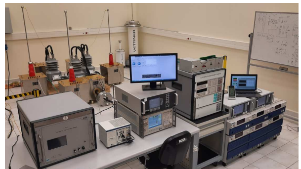
Fig. 9. A sample 3-phase combined transformer while testing.
