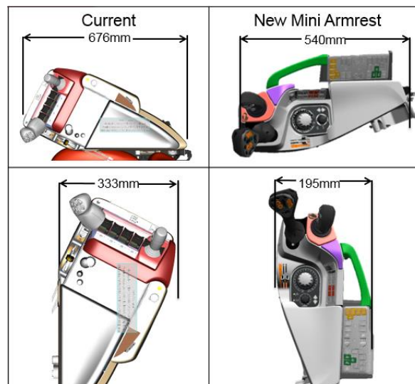
Fig. 12. UC1 compactness result: dimension comparison between the previous armrest and new compact-ergonomic armrest
