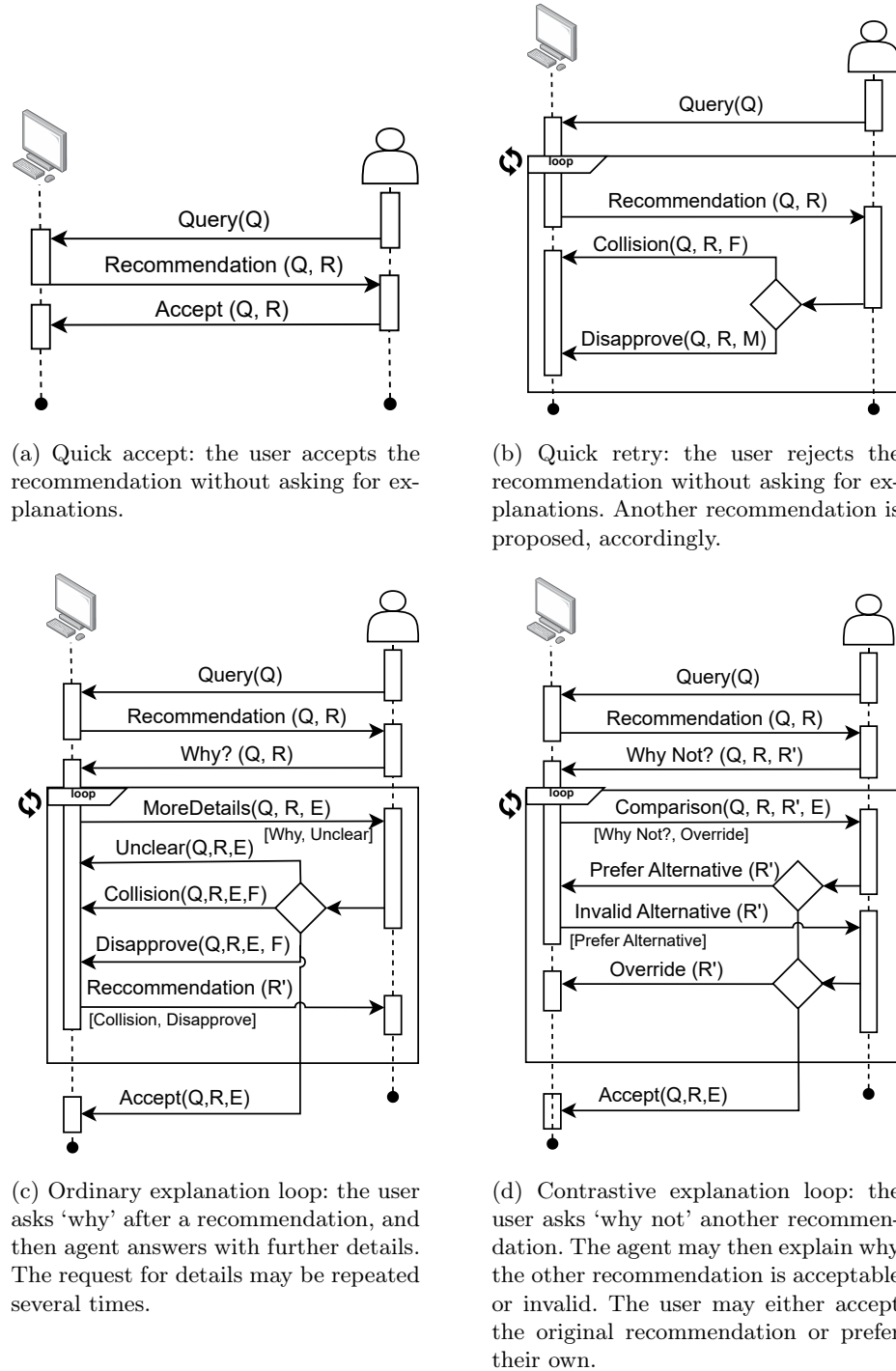
Fig. 3: Sequence diagrams describing most common scenarios of the protocol.
