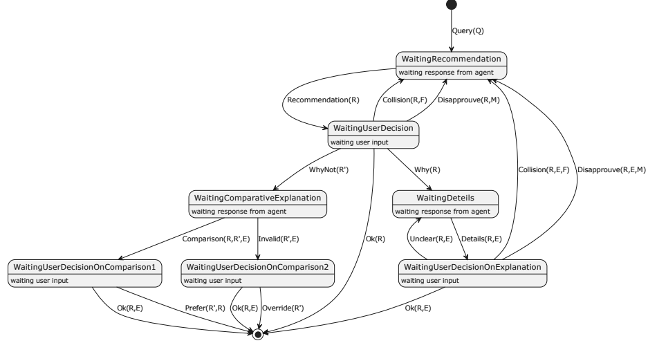
(a) Initiator-side state diagram.
