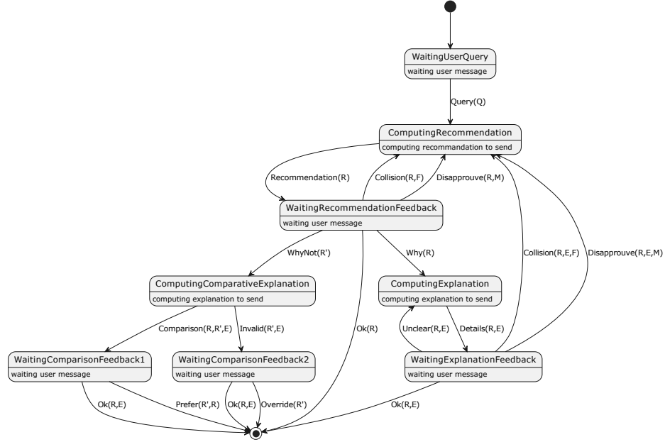
(b) Responder-side state diagram.
