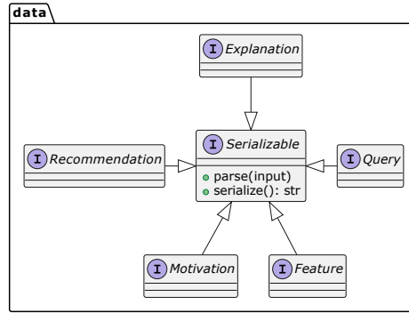
Fig. 5: Abstract classes for message payloads in PYXMAS.
