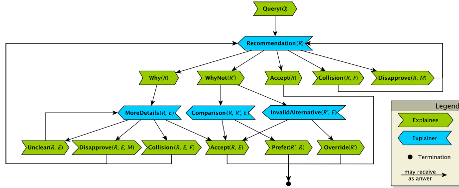
Fig. 2: Message communication diagram between an explainer agent (blue boxes) and an explaineer (green boxes). Each box represents a message. Each message is connected to the ones it can receive as reply.
