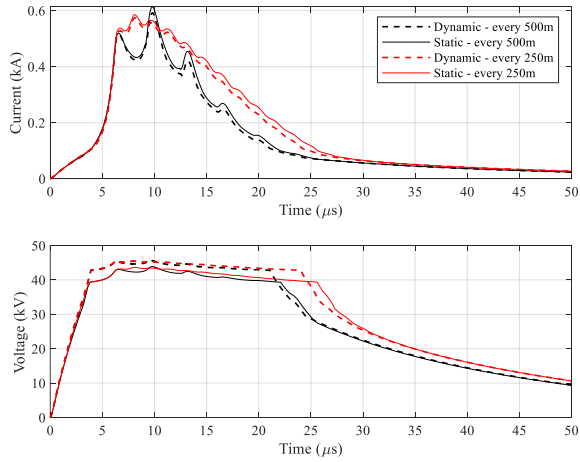
Fig. 6. SAs current and voltage due to an indirect first stroke varying the SAs distance. Indirect first stroke - location x = 1000 m, y = 50 m.
