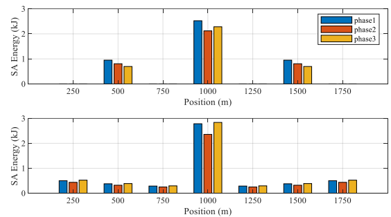
Fig. 11. Energy absorbed by SAs when installed every 500 m (top) and 250 m (bottom). Direct strike at x = 1000 m.
