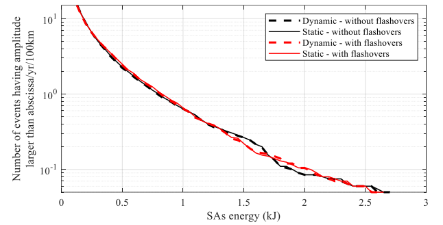
Fig. 13. Annual number of events causing a) currents and b) energy absorptions higher than the value in abscissa in at least one of the SAs (500 m spacing). Comparison between the static and dynamic model, with and without considering flashovers.
