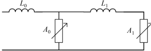
Fig. 1. Dynamic SA model proposed in [9].
