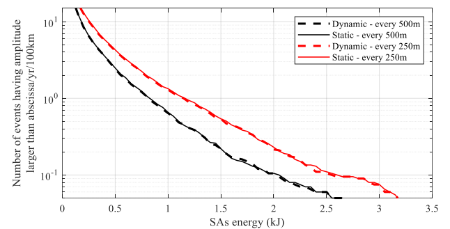
Fig. 14. Annual number of events causing a) currents and b) energy absorptions higher than the value in abscissa in at least one of the SAs. Comparison between different SAs spacing.
