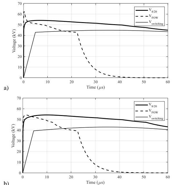
Fig. 3. Voltages across the SAs for the three different current waveforms of Fig. 2: a) dynamic model; b) static model.
