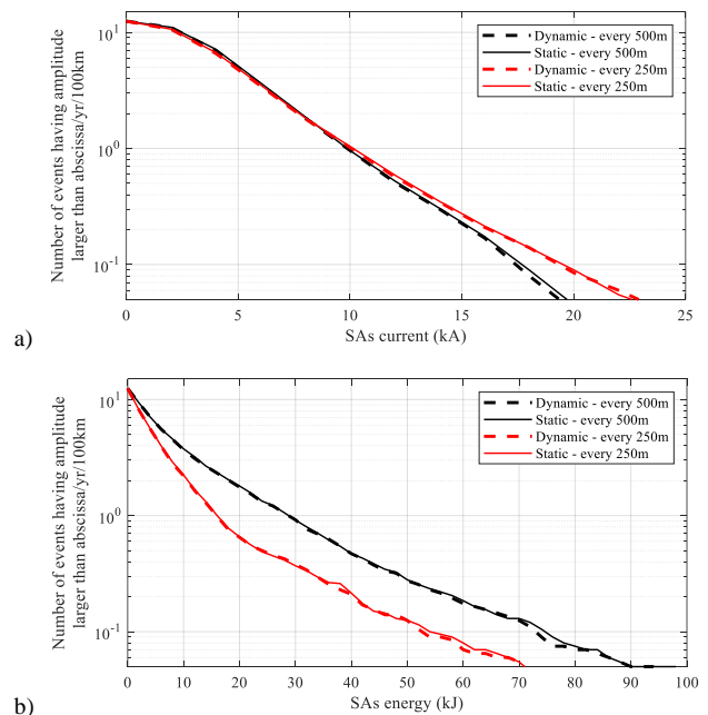
Fig. 18. Annual number of events originating a) currents and b) energy absorptions higher than the value in abscissa in at least one of the SAs. Comparison between different SAs spacing: 500 m and 250 m
