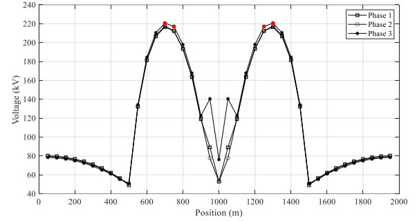
Fig. 9. Voltage peak amplitudes across insulators due to a first stroke on the shield-wire. Red markers indicate flashovers of phase-3 insulator. SAs installed every 500 m. Strike position = 1000 m.
