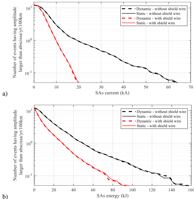
Fig. 16. Annual number of events originating a) currents and b) energy absorptions higher than the value in abscissa in at least one of the SAs (500 m spacing). Comparison between a line with and without shield wire.
