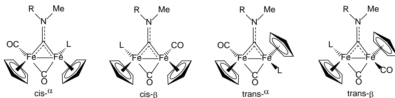
Figure 1. Possible isomers in diiron \mu -aminocarbyne derivatives ( \text{R} \neq \text{Me} , \text{L} = \text{anionic ligand} ).
