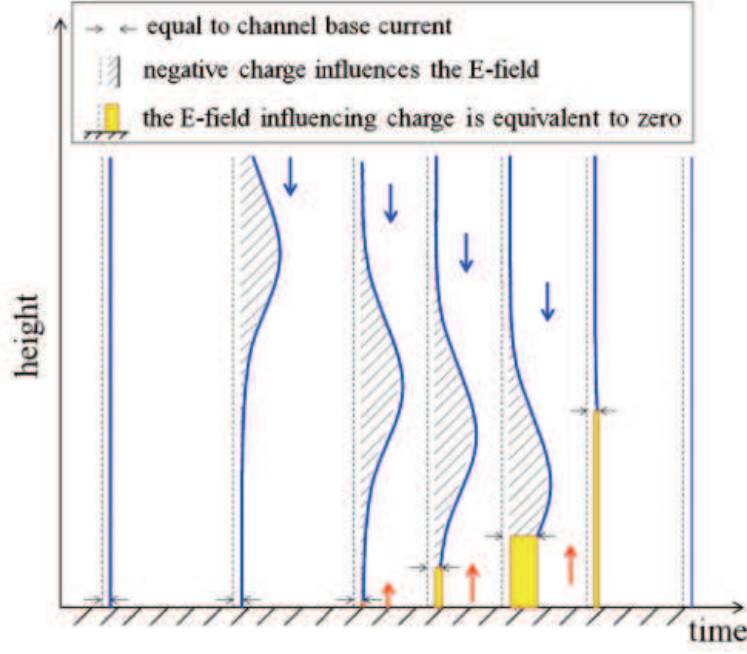
Figure 9. Diagram of the modified mechanism of M-component from Jiang et al. [38].
