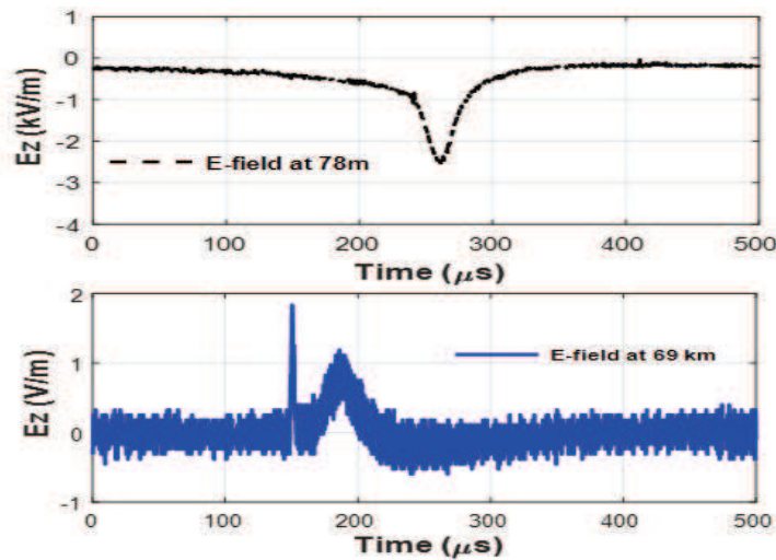
Figure 8. The simultaneously observed close and far electric fields in Li et al. [34].
