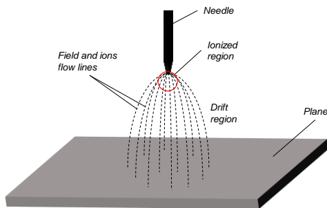
Fig. 1. Corona discharge in the point-to-plane geometry
