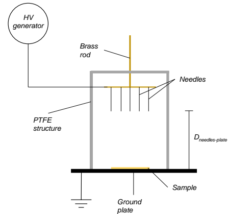
Fig. 2. Gridless corona poling set-up
