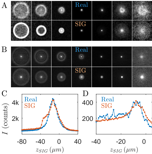
FIG. 3. Comparison between experimental and simulated particle image scans. (A) Real and synthetic images of 2- \mu\text{m} spheres taken with a 10 \times /0.3 objective lens. (B) Real and synthetic images of 1- \mu\text{m} spheres taken with a 63 \times /0.75 objective lens. (C) and (D) Corresponding maximum particle image intensity across the z direction.
