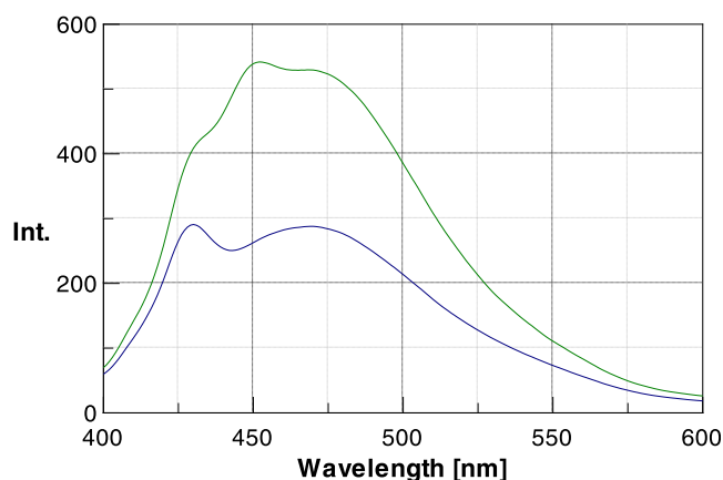
Figure 3. Fluorescence emission spectra of 23 (0.375 \mu M) in Gly–NaOH buffer (50 mM, pH 8.5) in the absence (blue line) and presence (green line) of preaggregated A \beta 42 (0.75 \mu M). [A \beta 42 ]/[ 23 ] = 2/1. \lambda_{\text{exc}} = 374 nm.
