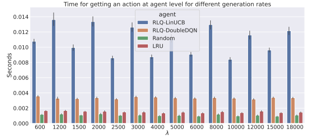
Fig. 5: Average time taken by the Agent to decide an action for different generation rates \lambda .
