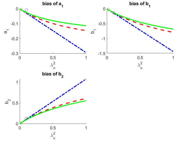
Fig. 2. Parameter biases versus \lambda_u^2 . The true biases ( \beta_t ) are shown with solid lines. The approximate biases ( \beta_1 ) are shown with dashed lines. The cruder approximate biases ( \beta_2 ) are shown with dashdotted lines. The circles show the empirical biases obtained by the Monte Carlo simulations from 100 realizations of length 1000. The value of the parameter \delta is \delta = 0.1 .
