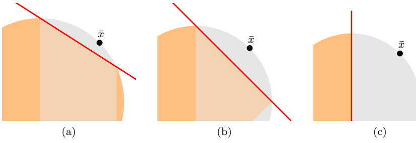
Fig. 3: Split cuts (in red) obtained with the polar normalization.
