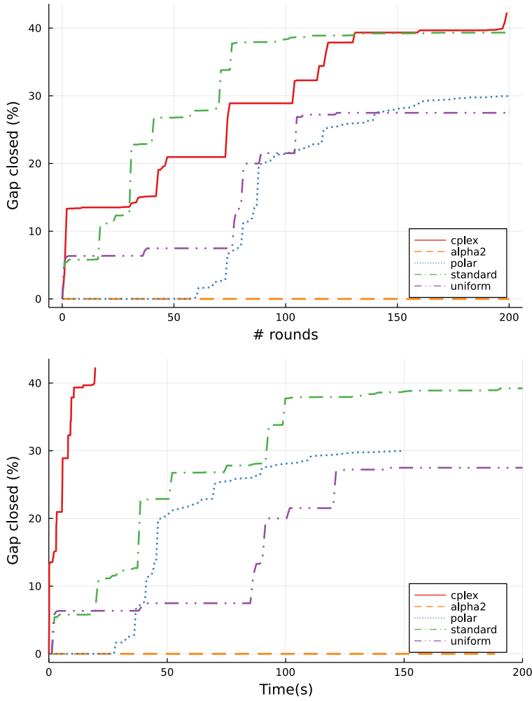
Fig. 9: Instance t1s4 : gap closed per round (top) and time (bottom)
