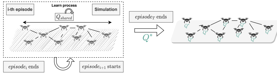
Fig. 2: Reinforcement Learning schema used in our simulations. The learning algorithm is applied at simulation time (for T episodes) improving a shared Q table. At the deployment time then, the agents exploit a local copy of the optimal Q^* table found by learning.
