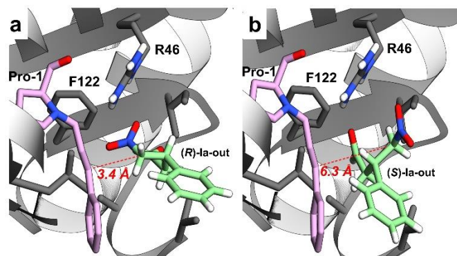
Figure 7. a) Docking of ( R )- 1a in the active site of Pp-4OT-F3: binding energy: 4.00 Kcal mol -1 . b) Docking of ( S )- 1a in the active site of Pp-4OT-F3: binding energy: 4.31 Kcal mol -1 . The iminium ion formed between Pro-1 and 2a is shown in purple while intermediate 1a is in green. The dashed red line shows the distance between the two reactive carbons for C-C bond formation. R46 is shown because it stabilizes 1a in the active site of the enzymes. For simplicity the ribbon of Pro-1 is not shown. All docking simulations performed with YASARA structure. UCSF Chimera software was used for visualization.
