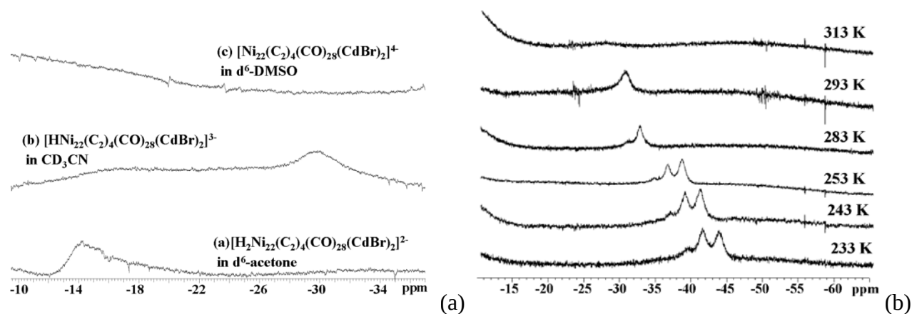
Fig. 20. (a) ^1\text{H} NMR spectra (400 MHz) recorded at 298 K of [\text{H}_{4-n}\text{Ni}_{22}(\text{C}_2)_4(\text{CO})_{28}(\text{CdBr})_2]^{n-} ( n = 2-4 ) in solvents of different basicity. (b) Variable temperature ^1\text{H} NMR spectra recorded at 600 MHz of [\text{H}\text{Ni}_{22}(\text{C}_2)_4(\text{CO})_{28}(\text{CdBr})_2]^{3-} in \text{CD}_3\text{CN} . Reproduced with permission from ref. 88.
