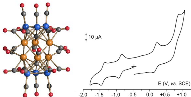
Fig. 7. (a) Molecular structure of [\text{Co}_8\text{Pt}_4\text{C}_2(\text{CO})_{24}]^{n-} ( n = 1,2 ). Co as blue sphere, disordered Co/Pt orange, C gray and O red. (b) Cyclic voltammetric response recorded at a glassy carbon electrode in THF solution of crystalline [\text{NMe}_3(\text{CH}_2\text{Ph})]_2[\text{Co}_8\text{Pt}_4\text{C}_2(\text{CO})_{24}] ( 1.2 \times 10^{-3} M). [\text{NBu}_4][\text{PF}_6] (0.2 M) supporting electrolyte. Scan rates 0.2 \text{ V s}^{-1} . Reproduced with permission from ref. 89.
