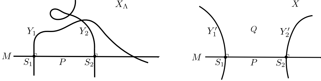
FIGURE 1. A schematic picture of X_\Lambda (left) and of its finite cover X (right) with their horizontal and vertical hypersurfaces. A piece P of M embeds “nicely” in a piece Q of X . Each Y'_i finitely covers Y_i .
