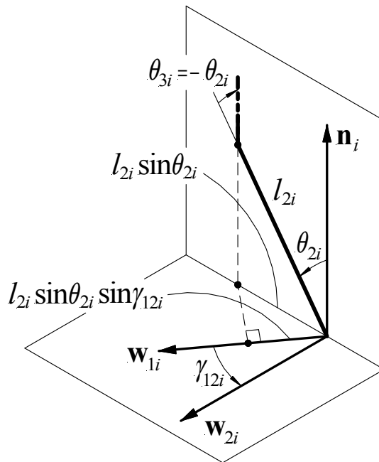
Fig. 18: Platform displacement along the constant direction \mathbf{w}_{1i} in a fully-isotropic T_5'' TPM.
