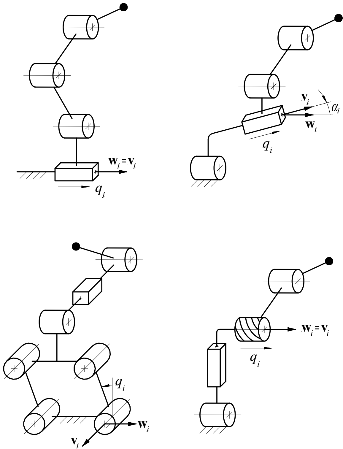
Fig. 9: Examples of architectures of type I fully-isotropic T_4 TPM legs.
