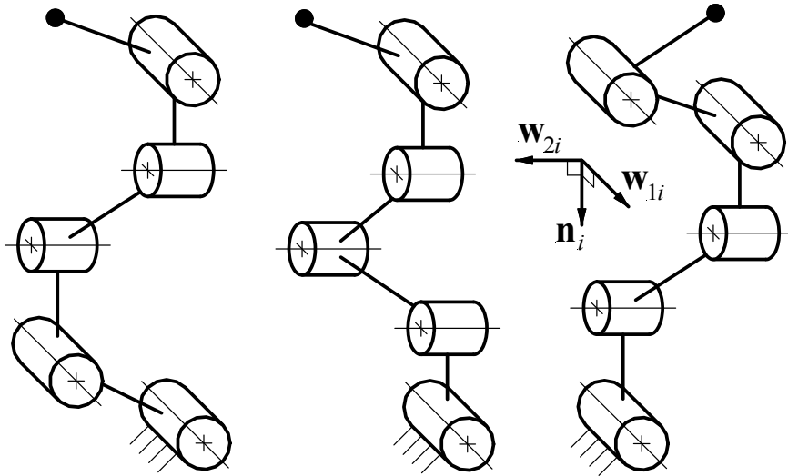
Fig. 6: Type T_5'' legs with five R-pairs.
