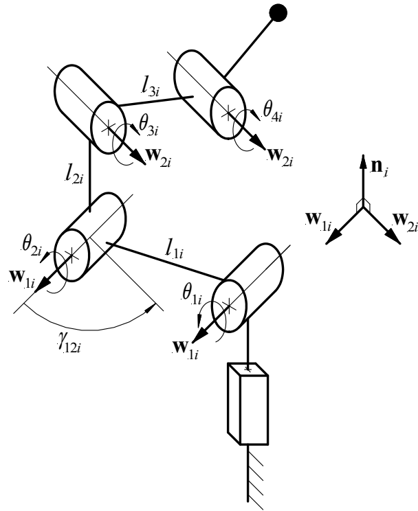
Fig. 3: A type T_5' leg with four R-pairs.
