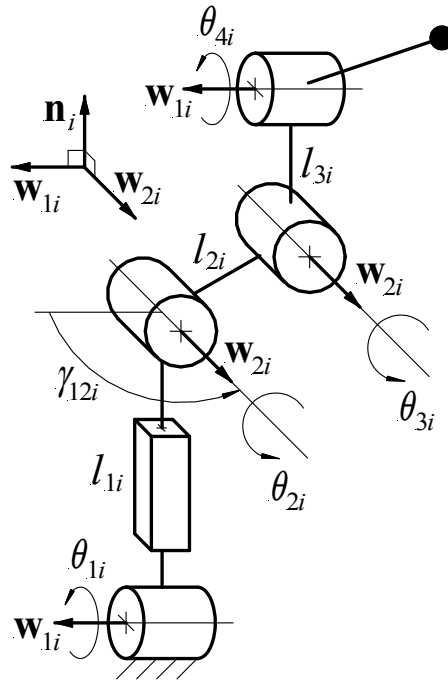
Fig. 5: A type T_5'' leg with four R-pairs.
