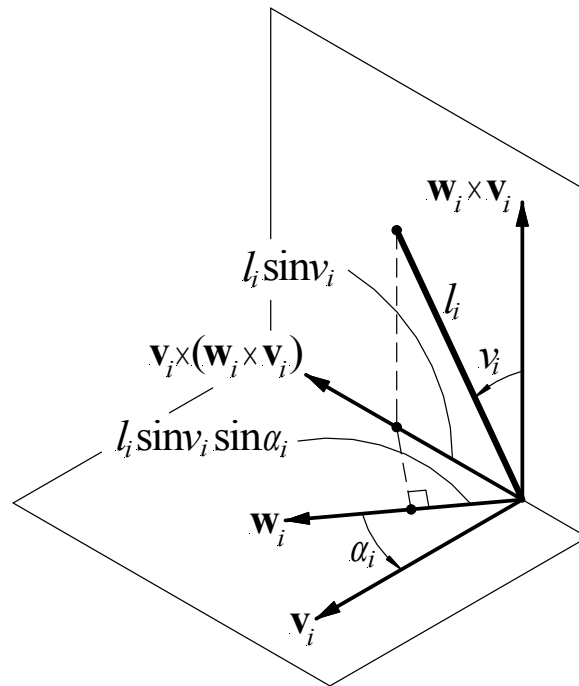
Fig. 8: Motion of one of the cranks of a parallelogram that permits, in a type T_4 leg, the platform's movement out of the plane perpendicular to \mathbf{w}_i .
