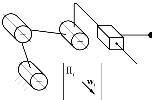
Fig. 2: A type T_4 leg with three R-pairs.
