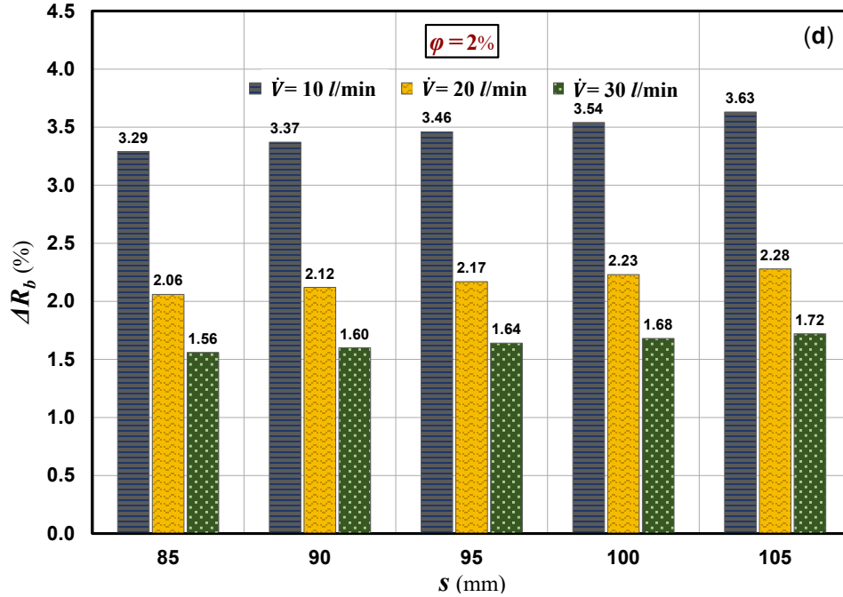
Fig. 13. Combined effects of the shank spacing ( s ) and the volume fraction of nanofluids on the decrement percentage of thermal resistance ( \Delta R_b ) at different volume flow rates: \phi=0.5\% (a)- \phi=2.0\% (d).
