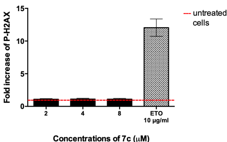
Figure 10. Relative expression of P-H2AX following 5h treatment of Jurkat cells with increasing concentrations of 7c . Etoposide (ETO) 10μg/mL was used as positive control. **p< 0.01 versus untreated cells.
