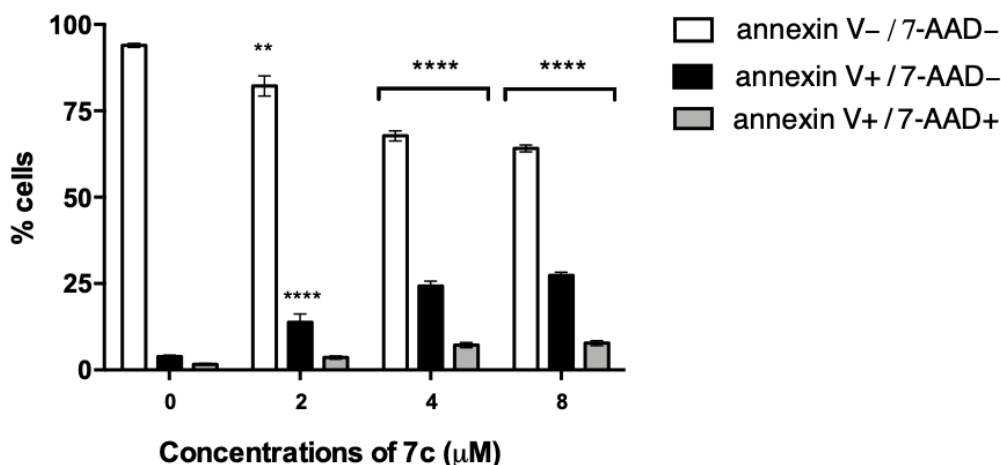
Figure 3. Percentage (%) of viable (annexin V - /7-AAD - ), early apoptotic (annexin V + /7-AAD - ), and late apoptotic or necrotic (annexin V + /7-AAD + ) cells after 24h treatment of Jurkat cells with increasing concentrations of 7c . ** p < 0.01; **** p < 0.0001 versus untreated cells.
