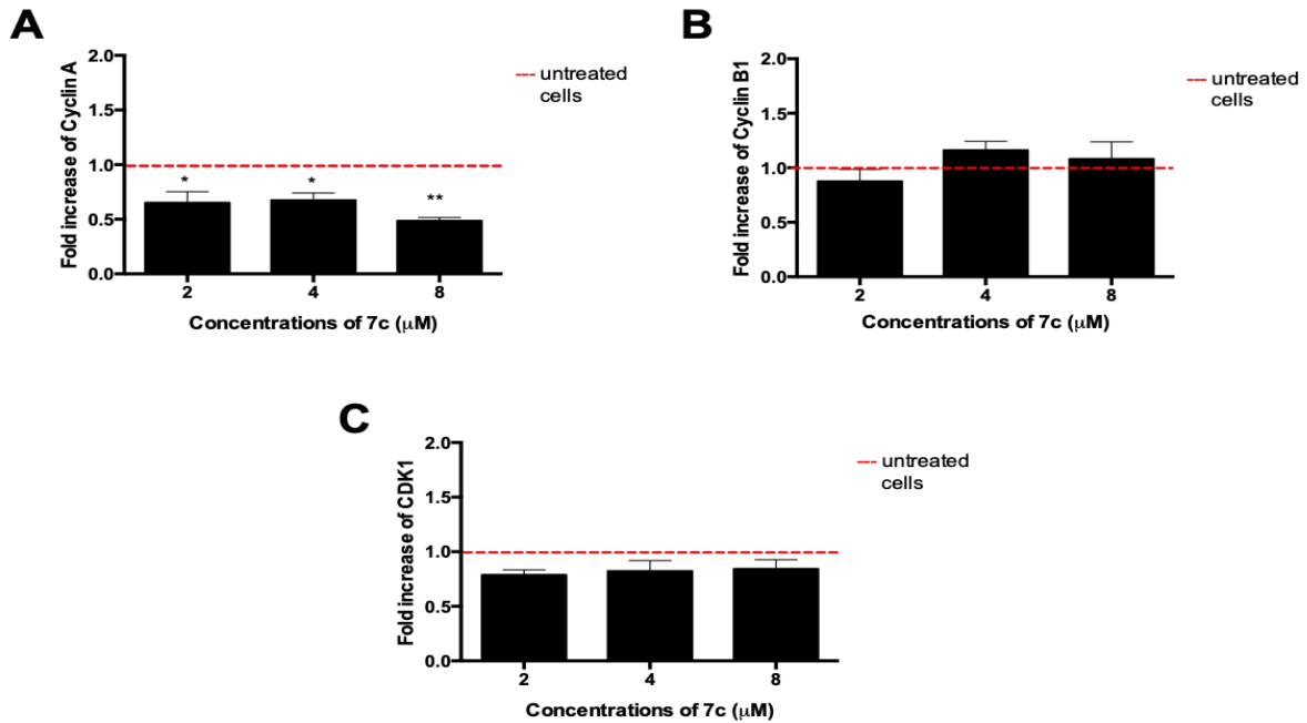
Figure 8. Expression of cyclin A (A), cyclin B1 (B), and CDK1 (C), indicated as fold increase versus untreated cells, following 24h treatment of Jurkat cells with increasing concentration of 7c. *p< 0.05; **p< 0.01 versus untreated cells.
