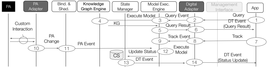
Fig. 8. Interaction of an external application with the DT: query and track.
