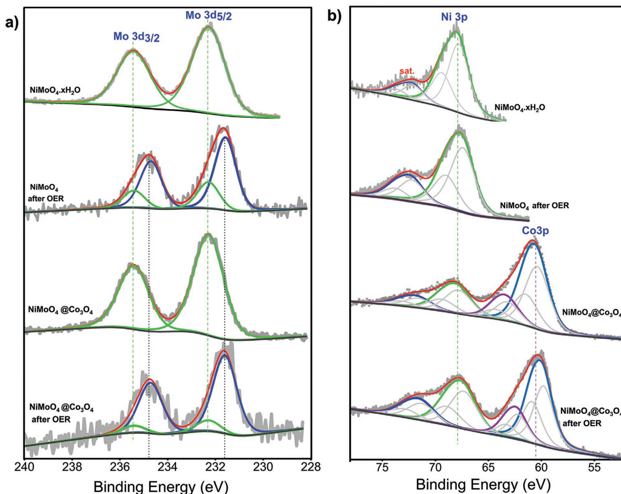
Figure 7. XPS spectra of the as-prepared catalysts. a) Mo 3d spectra for hydrous NiMoO 4 before and after catalysis, and Mo 3d spectra of NiMoO 4 @Co 3 O 4 before and after catalysis. b) Ni 3p spectra for NiMoO 4 before and after catalysis, and Ni 3p and Co 3p spectra for NiMoO 4 @Co 3 O 4 before and after catalysis. All the spectra were acquired using 690 eV p-polarized photons.
