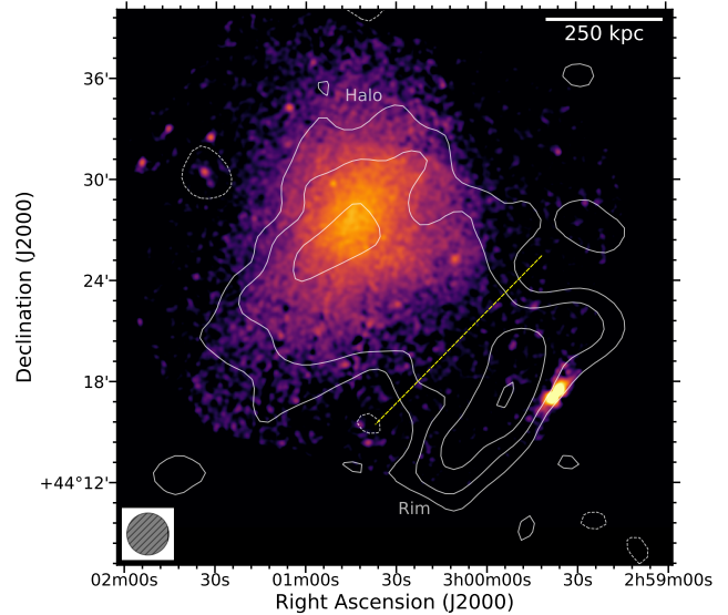
Figure 2. XMM-Newton image in the 0.5–2.0 keV with overlaid the LOFAR source-subtracted contours at 150'' resolution of Fig. 1. The dashed yellow line separates the halo and Rim regions.
