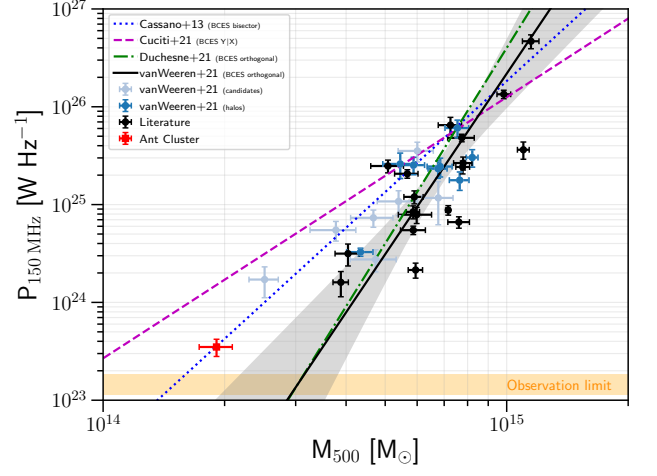
Figure 4. The position of the Ant Cluster in the P_{150} - M_{500} relation of van Weeren et al. (2020). The reference scaling relations reported by Cassano et al. (2013); Cuciti et al. (2021b); Duchesne et al. (2021), rescaled to 150 MHz adopting \alpha = 1.3 , are also shown. The orange horizontal region marks the detection limit for our LOFAR 180'' image.
