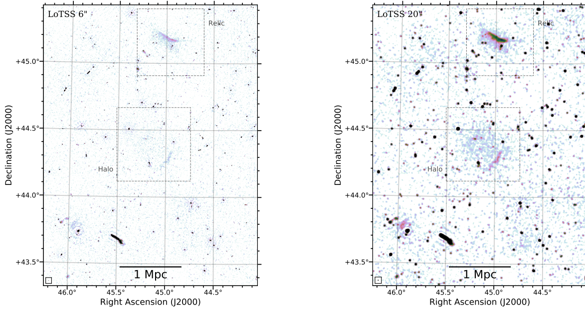
Figure 5. LoTSS images at 6'' (left) and 20'' (right) resolution and with a noise of 93 and 160 \mu\text{Jy beam}^{-1} , respectively. The FoV and dashed boxes are the same of the left panel of Fig. 1.
