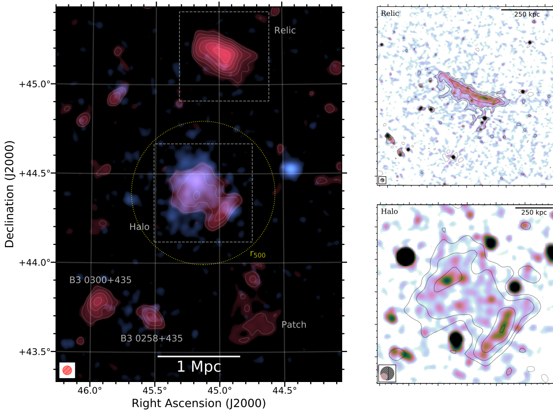
Figure 1. Left panel: composite radio (LOFAR 120–168 MHz, red) + X-ray (ROSAT 0.1–2.4 keV, blue) image of a 1.6^\circ \times 2.1^\circ field centered on the Ant Cluster. The LOFAR image has a resolution of 180'' and was obtained after subtracting discrete sources in the uv -plane. The dashed boxes mark the regions where we improved the calibration of LoTSS data. Right panels: zoom-in of the (reprocessed) relic and halo regions. Colors indicate the images at 15'' and 75'' resolution for the relic and halo, respectively. Contours show the discrete source-subtracted emission from images with double beam width. Contours are spaced by a factor of 2 starting from 2.5\sigma . The -2.5\sigma contour is reported with dashed lines. The beam of the radio images is shown in the bottom left corners. The noise level and resolution are listed in Tab. 1.
