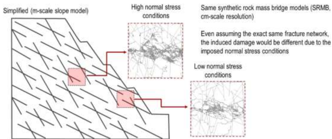
Fig. 9 Example of how progressive rock mass damage would change depending on the location of the rock mass bridge and the imposed normal stress conditions
