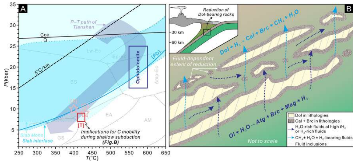
Fig. 9. (A) Summary of abiotic \text{CH}_4 formation through dolomite reduction in ophidolomites during exhumation of the Chinese southwestern Tianshan. The P T constraints for HP ophidolomites in the Tianshan are from Peng et al. (2020). The red rectangle [T] displays P T conditions for the onset of dolomite reduction, inferred from retrograde serpentinization in the Tianshan (Li et al., 2007, 2010). For comparison, P T estimates for carbonate reduction during shallow subduction in Alpine Corsica [C] (Malvoison et al., 2012; Galvez et al., 2013a, b) and the Italian Alps [A] (Vitale Brovarone et al., 2017; Giuntoli et al., 2020) are shown. The P T path of the Tianshan is from Tan et al. (2017). The cyan and light cyan areas represent the modelled prograde P T paths of subduction zones at the slab interface and slab Moho (7 km beneath the slab surface; Syracuse et al., 2010). The sky blue solid curve (PD) shows the global average range of prograde P T paths from subduction related metamorphic rocks (Penniston Dorland et al., 2015). Facies boundaries and abbreviations are from Liou et al. (2004). (B) General model showing abiotic \text{CH}_4 production through dolomite reduction during shallow subduction. Due to uncertainties in the scale and extent of serpentinization in subducted slabs (Li et al., 2007, 2010; Vitale Brovarone et al., 2017, 2020; Lazar, 2020), dashed arrow lines represent fluid migration pathways instead of the steady fluid flow. The extent of alteration is dependent on the infiltration of the reactive reduced fluids. Possible \text{CH}_4 \text{H}_2 generating reactions are listed but without stoichiometric numbers. Figure is not to scale.
