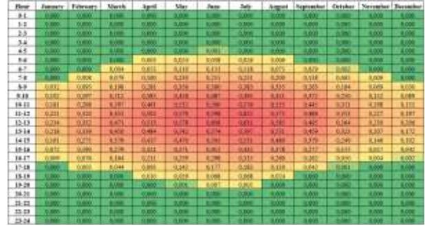
Figure 4. The monthly average hourly profile for a photovoltaic plant in Ravenna (kWh/kWp)
