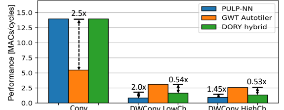
Fig. 9. Comparison between HWC, CHW, and DORY layers layout. Different kernels are explored.
