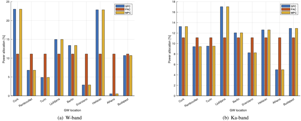
Fig. 10. Percentage of power allocated per GW with SPC, PAC, and MPC in W-band (left) and Ka-band (right), p = 10^{-3} (99.9% availability).
