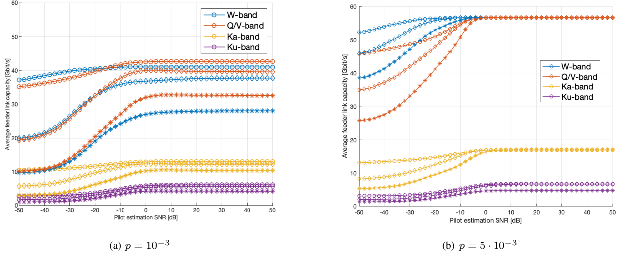
Fig. 9. Average feeder link capacity with PAC (circle), SPC (diamond), and MPC (asterisk) with MMSE precoding as a function of the pilot estimation SNR.
