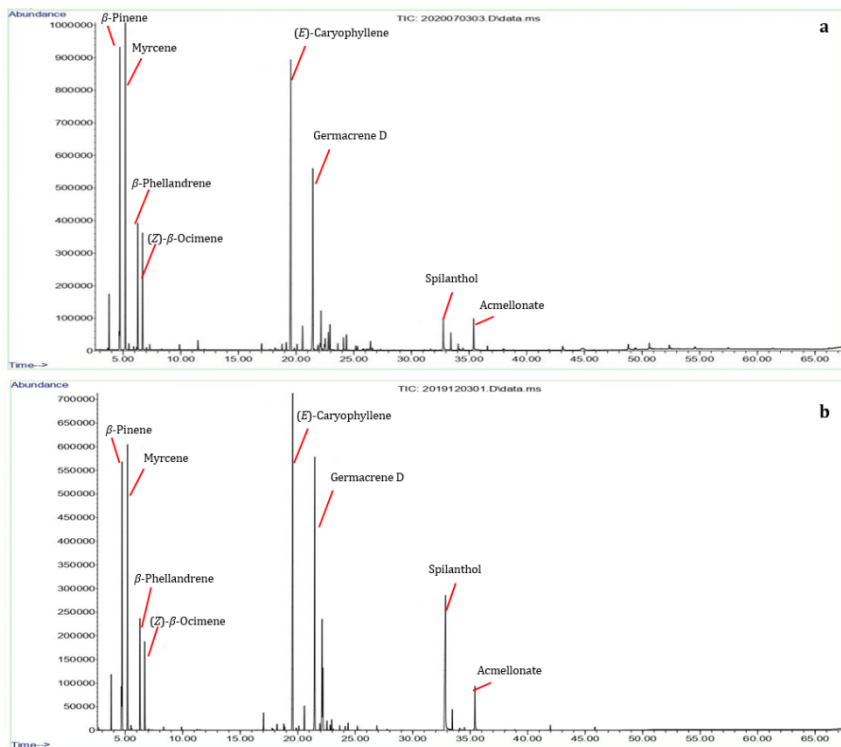
Fig. 1SM. GC-MS chromatograms of Acmella oleracea essential oil obtained by hydrodistillation (HD, a) and microwave-assisted extraction (MAE, b).
