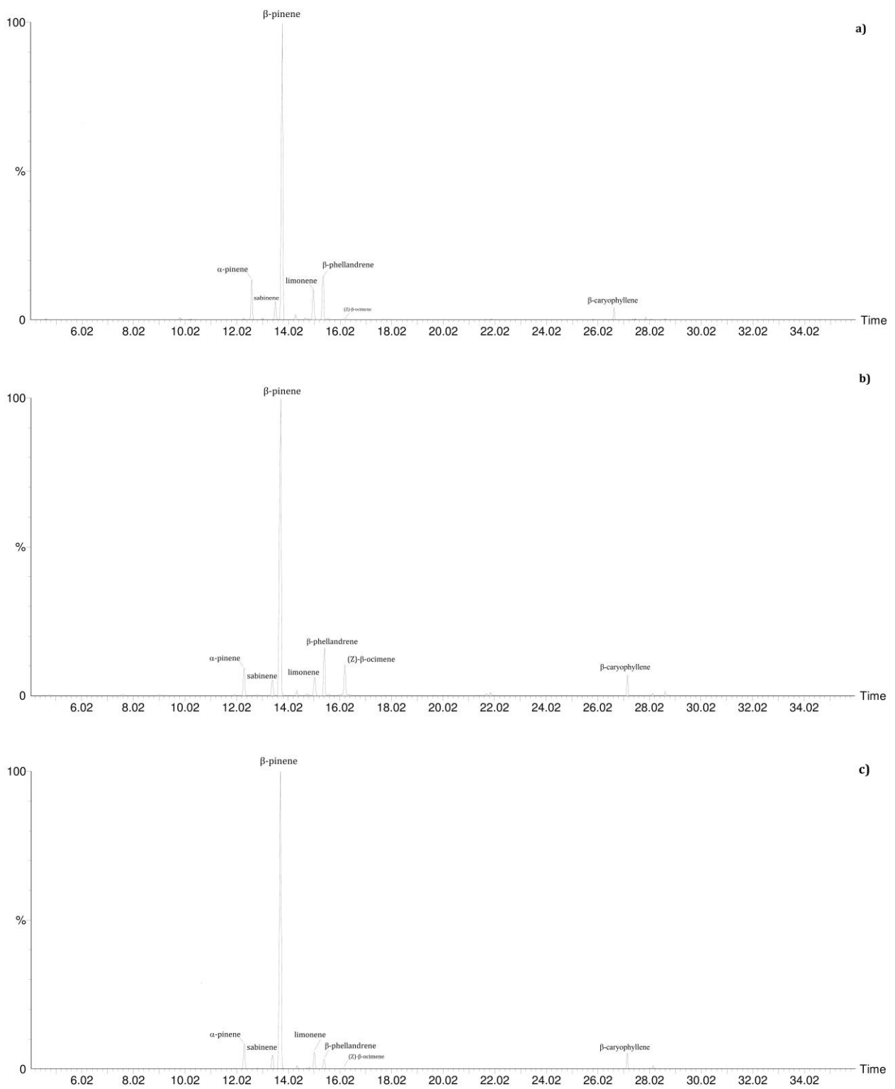
Fig. 4. GC-MS chemical fingerprint of the vapour phase of Acemella oleracea essential oil (a), its nanoemulsion at time 0 (b), and after 4 months of storage (c).
