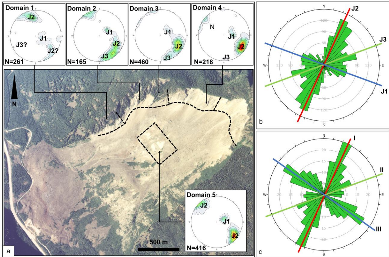
Fig. 11 Overview of the outcrop-scale second order discontinuity mapping performed at the Hope Slide. a: summary of the results from the TDP discontinuity mapping described in Donati et al. (2013). All the stereonet are equal angle, lower hemisphere projections. On the aerial photograph, the dashed lines outline the boundaries of the structural domains derived from the discontinuity mapping (photograph 1996, courtesy of Province of British Columbia, roll BCC96082, frame 19). b: rosette diagram that includes the mapped discontinuities. The orientations of the principal discontinuity sets identified are highlighted. c: rosette diagram obtained from the slope-scale lineaments. Note the similarities with the discontinuity set orientations in b.
