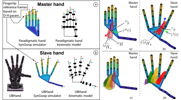
Fig. 4. (a) Master hand (paradigmatic hand) and (b) slave hand (UBHand).
