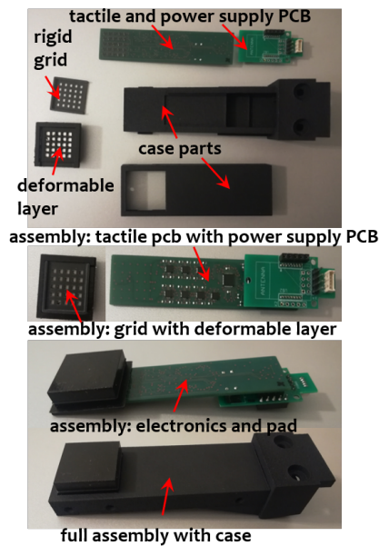
Fig. 1. Detailed view of the sensorized finger.
