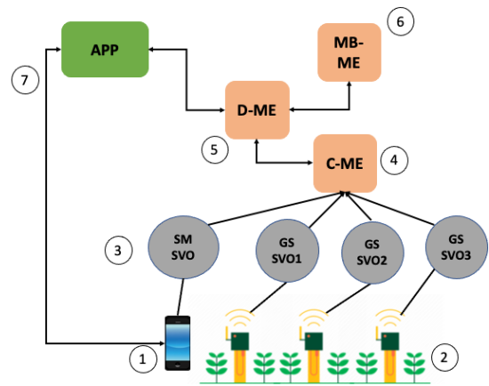
Fig. 1. The FruGar System's architecture.
