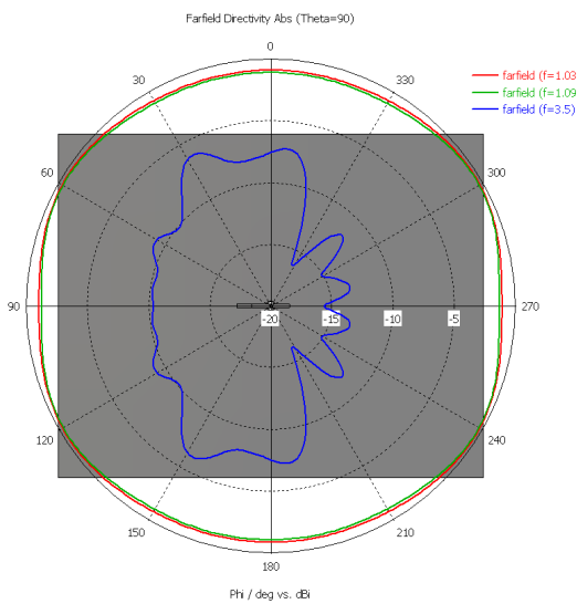
(c) XY, H-plane
