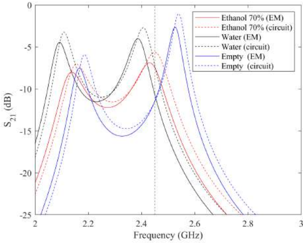
Fig. 25. Transmission coefficient of the filter for the different fluids filling the channel: comparison between full-wave and circuital simulations.
