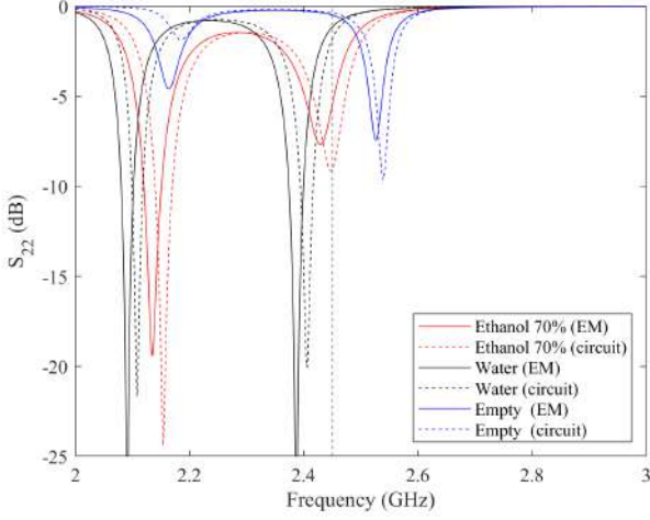
Fig. 24. Reflection coefficient of the filter output port for the different fluids filling the channel: comparison between full-wave and circuital simulations.
