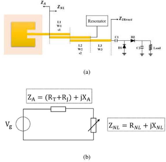
Fig. 17. (a) Circuit schematic of the designed filtenna loaded by the rectifier and (b) its equivalent representation, consisting of a Thevenin equivalent of the receiving antenna loaded by a nonlinear complex impedance.
