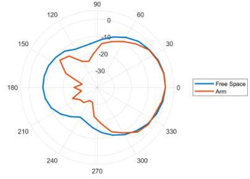
Fig. 29. Radiation diagram for the designed patch antenna: the blue curve represents a measurement in air and the red one when the antenna is placed on an arm.
