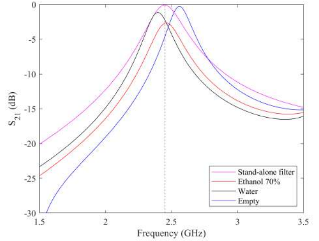
Fig. 14. Predicted transmission coefficients of the reference filter and the loaded ones, with the channel filled with the different fluids.
