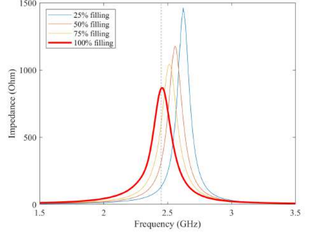
Fig. 6. Frequency behavior of the real part of the stub input impedance for different filling percentages.
