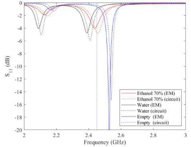
Fig. 23. Reflection coefficient of the filter input port for the different fluids filling the channel: comparison between full-wave and circuital simulations.
