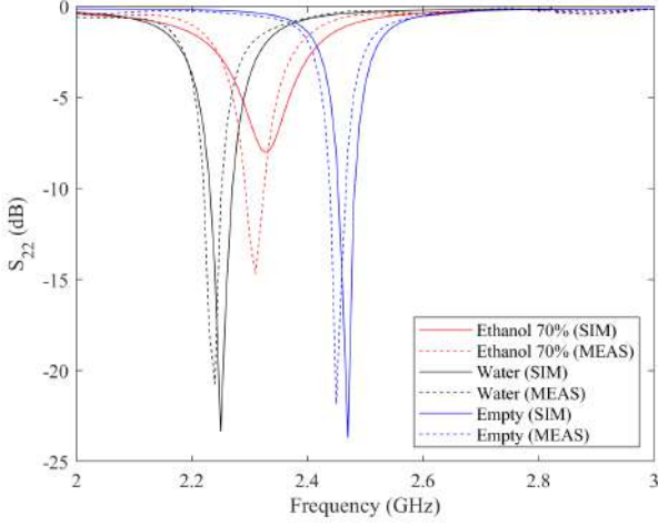
Fig. 32. Reflection coefficient at the filter output port: full-wave simulated and measurement results for the different fluid filling the channel.
