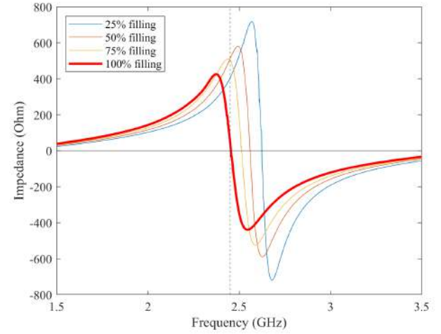
Fig. 7. Frequency behavior of the imaginary part of the stub input impedance for different filling percentages.
