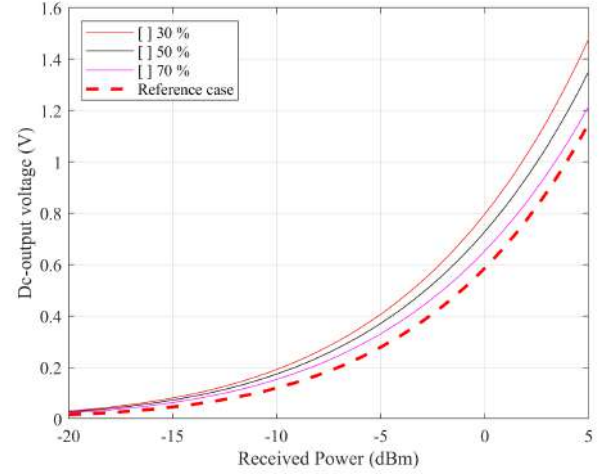
Fig. 26. Dc-output voltage levels for a half-filled channel with different ethanol concentration, compared to the reference case.
