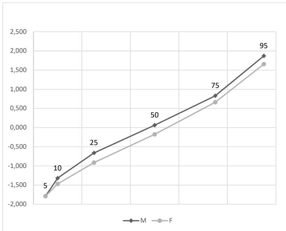
FIGURE 1. Percentile distribution of performance based on Rasch model by gender, grade 5.
