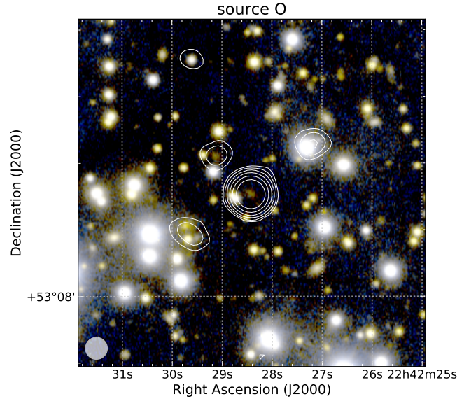
Figure 12. Subaru g-gi-i optical image of source O (Dawson et al. 2015; Jee et al. 2015). 1–4 GHz total intensity radio contours at 2.5'' resolution are overlaid at levels of 3\sigma_{\text{rms}} = \sqrt{(1, 4, 16, \dots)} , with \sigma_{\text{rms}} = 5.6 \mu\text{Jy beam}^{-1} the map noise (Di Gennaro et al. 2018).
