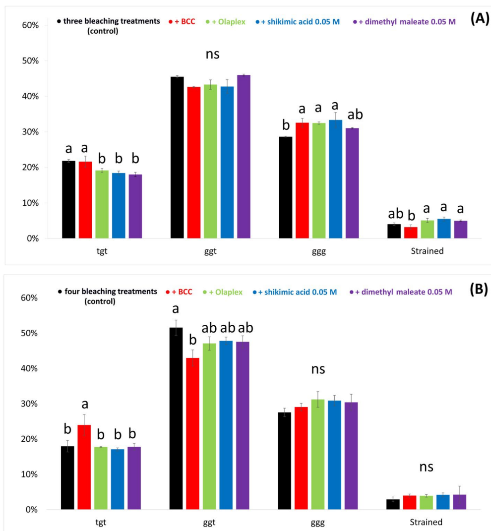
Fig. 5. (A) Percentages (average \pm standard deviation) of strained, gauche-gauche-gauche (ggg), gauche-gauche-trans (ggt) and trans-gauche-trans (tgt) C_{\alpha} - C_{\beta} -S-S- C_{\beta} - C_{\alpha} conformations as obtained by the curve fitting of the Raman S-S stretching range of: (A) the hair locks bleached three times and after treatment with BCC, Olaplex, shikimic acid 0.05 and dimethyl maleate 0.05 M; (B) the hair locks bleached four times, and after treatment with BCC, Olaplex, shikimic acid 0.05 and dimethyl maleate 0.05 M. For each conformation, different letters on histogram bars represent statistically significant differences; ns = not significant.
