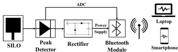
Fig. 2. Block diagram of the entire system for simultaneous energy harvesting and breath detection.
