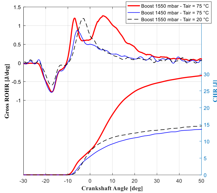
FIGURE 5: ROHR AND CHR TRACES FOR 3 TESTS RUN AT 2000 rpm, SOI EQUAL TO 26 deg BTDC, ALL RUN INJECTING 4 mg/stroke AT 300 bar AND CHANGING THE INTAKE CONDITIONS (PRESSURE AND TEMPERATURE).
