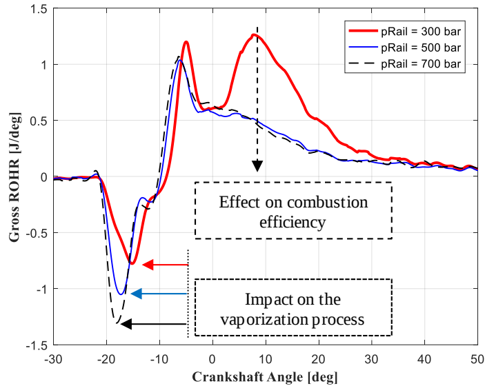
FIGURE 6: ROHR TRACES FOR 3 TESTS RUN AT 2000 rpm, SOI EQUAL TO 26 deg BTDC, ALL RUN INJECTING 4 mg/stroke AND CHANGING THE FUEL PRESSURE (INTAKE CONDITIONS ARE KEPT APPROXIMATELY CONSTANT).
