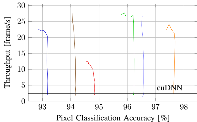
Fig. 9. Evaluation of the throughput-accuracy trade-off for all 6 video sequences.
