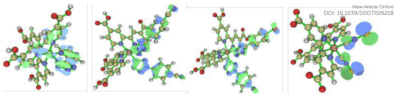
Figure 6. HSOMO isodensity surfaces for the D1 , D3 and D4 dyes in the oxidized form compared with N719 (left to right respectively).
