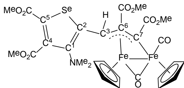
Chart 7. Structure of 6a .
