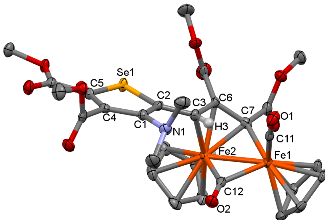
Figure 1. Molecular structure of 6a . Displacement ellipsoids are at the 30% probability level. H-atoms, except H(3), have been omitted for clarity.
