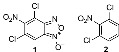
Figure 1. Structures of 4,6-dichloro-5-nitrobenzofuroxan ( 1 ) and 1,3-dichloro-2-nitrobenzene ( 2 ).
