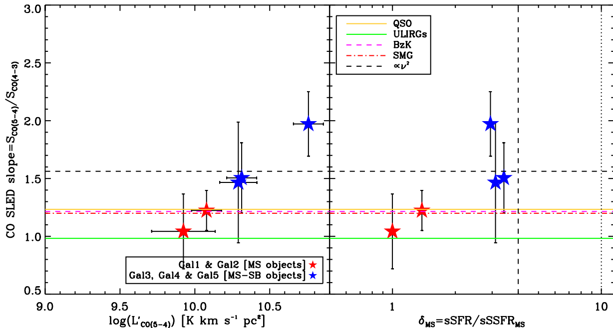
Figure 5. The CO Spectral Line Energy Distribution (SLED) slope between CO(5-4) and CO(4-3), defined as S_{CO(5-4)}/S_{CO(4-3)} , as a function of the CO(5-4) luminosity L'_{CO(5-4)} (left panel) and of \delta_{MS} (right panel: for clarity here we show the value obtained using the SFR derived by MAGPHYS only, but the result does not change if we use the SFR derived from the FIR), for the five galaxies in the sample. The colored horizontal lines show the average SLED slope for different classes of objects: continuous yellow for the median of the QSOs from Carilli & Walter (their Figure 4); dot-dashed red for SMGs (Bothwell et al. 2013); dashed magenta for BzK (Daddi et al. 2015); and green for local ULIRGs (Papadopoulos et al. 2012). The dashed horizontal line shows the slope for the case of constant brightness temperature on the Rayleigh-Jeans scale, i.e., S \propto \nu^2 . The vertical lines in the left panel highlight the loci 4x and 10x above the MS. The two galaxies that are closer to the MS (Gal1 & Gal2) are shown with red stars, while the three that are at the boundary between MS and starbursts are shown in blue. Error bars are estimated by propagating the errors on the individual fluxes to the ratio.
