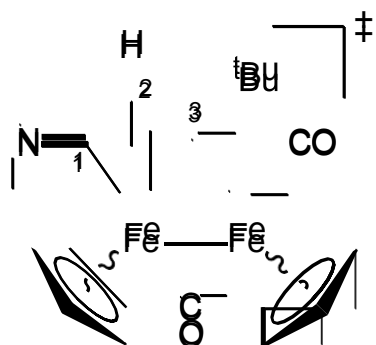
Chart 5. Structure of [2j] + .
