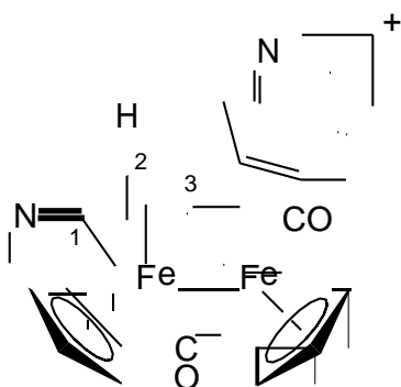
Chart 6. Structure of [2l] + .
