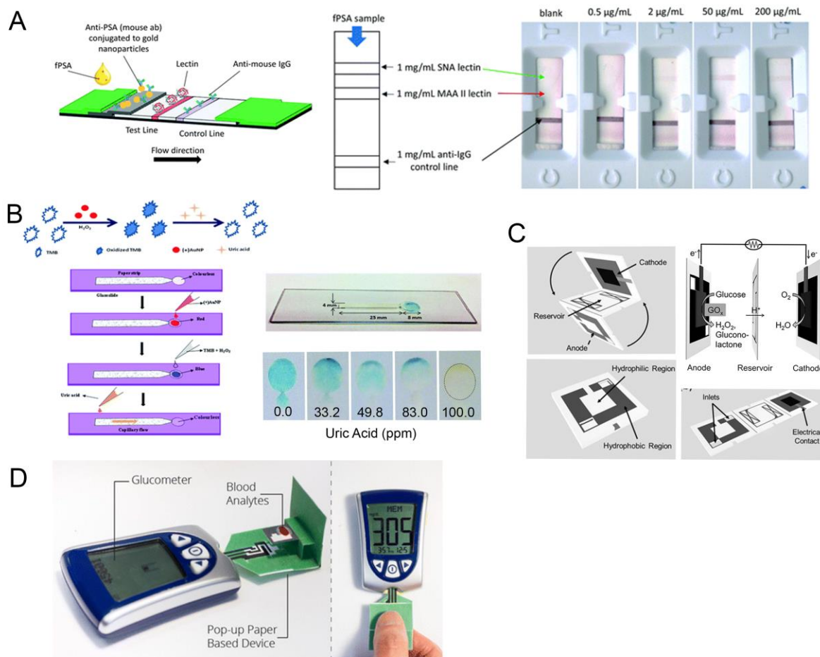
Fig. 2. Paper-based devices for diagnostic applications. (A) Lectin-based lateral flow assay for the detection of the prostate specific antigen. Reproduced from ref. 91 with permission
