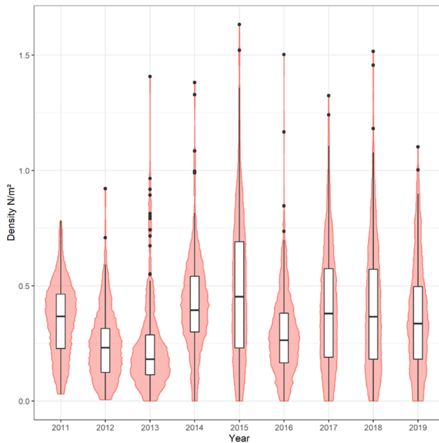
Figure 2: FU 3&4 (Skagerrak/Kattegat) times series of Nephrops burrow density (The horizontal lines represents the medians, the boxes are the inter quartile range, the shaded areas show the kernel probability densities of the data at different values and the black dots are potential outliers).
