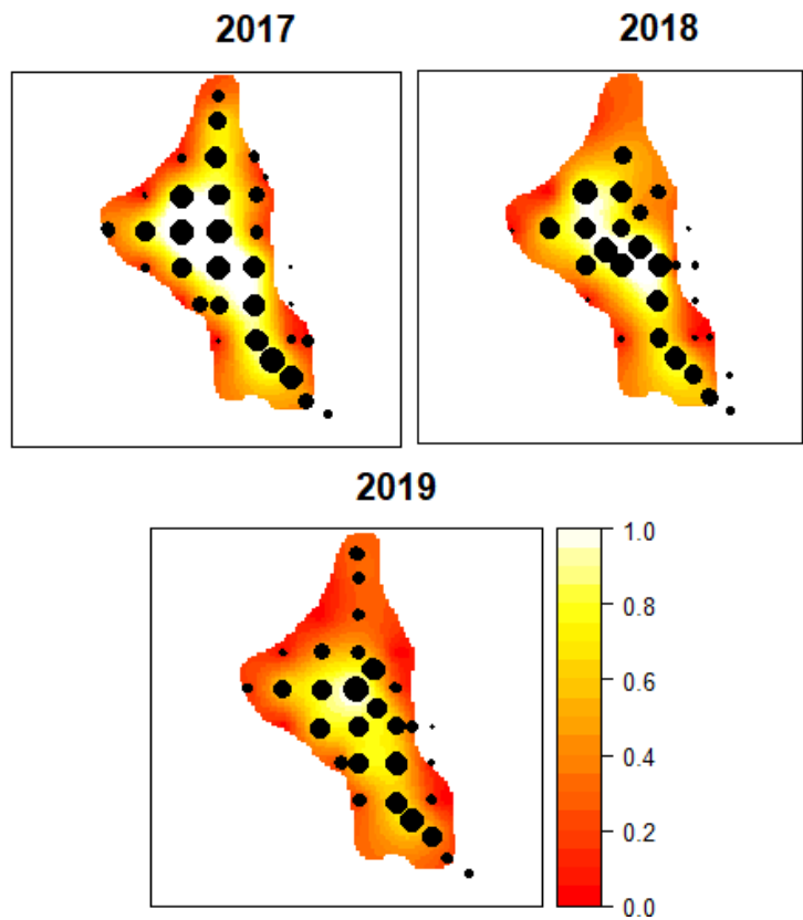
Figure 6 – Geostatistical outputs 2017 – 2019, maps of Nephrops density distribution (m 2 ).
