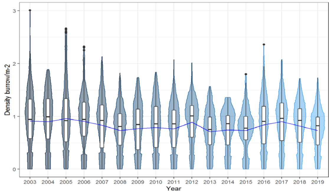
Figure 2: Times series of adjusted burrow density (Violin and box plot).
