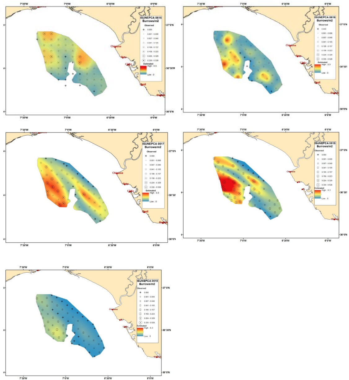
Figure 1: Gulf of Cadiz (FU 30). Bubble plot of the burrow density observations overlaid on a head map krigged burrow density surface for UWT survey series (2015-2019). Station positions with zero density are indicated using a +.
