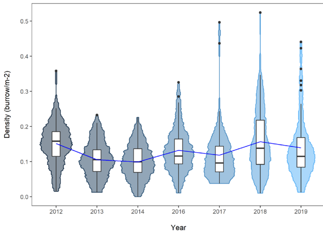
Figure 5. Porcupine Bank 2019. Violin and box plot of adjusted burrow density distributions by year for the available time series. The blue line indicates the mean density over time. The horizontal black line represents the median, white box is the inter quartile range, the black vertical line is the range and the black dots are outliers. No UWTV survey in 2015.
