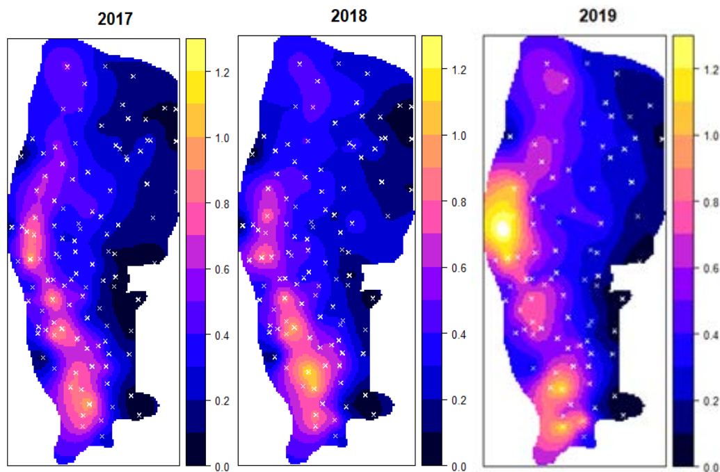
Figure 3 – Geostatistical outputs 2017 – 2019, maps of Nephrops density distribution (m 2 ).
