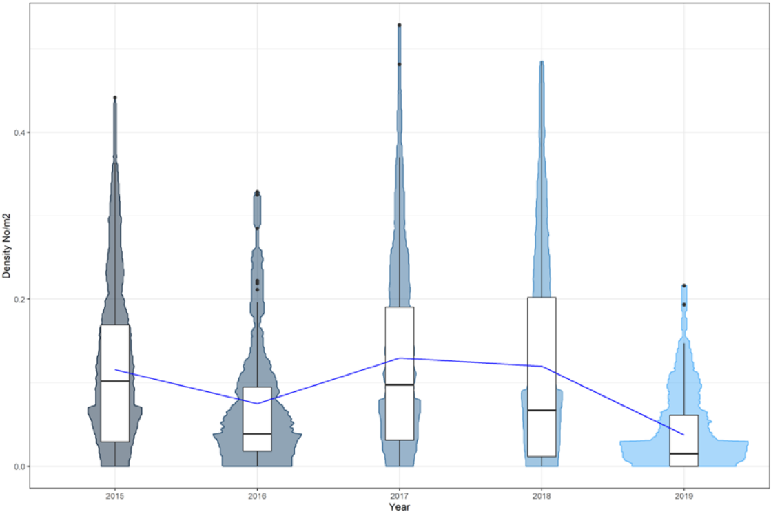
Figure 2: Gulf of Cadiz (FU 30) times series of adjusted burrow density (Violin and box plot).
