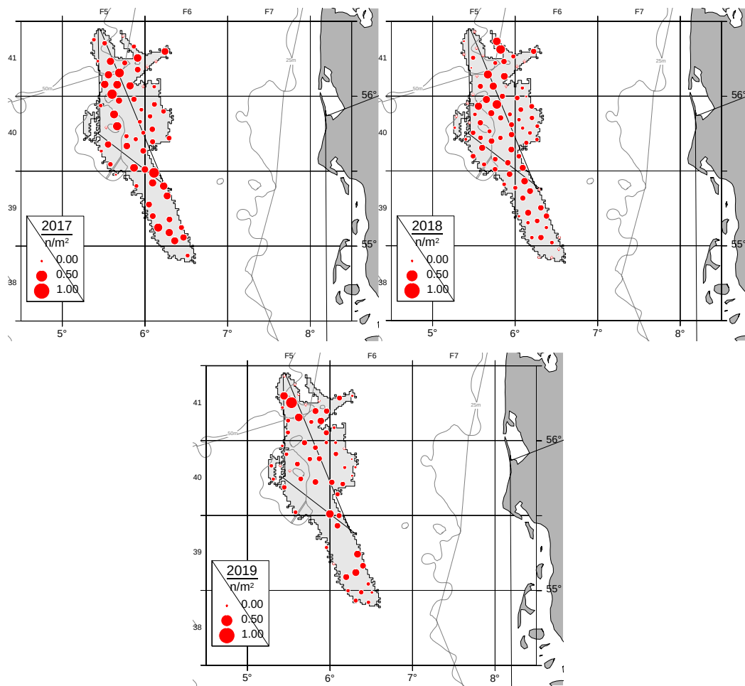
Figure 1: FU 33 (Off Horns Rev) Nephrops burrow density by station for each year.
