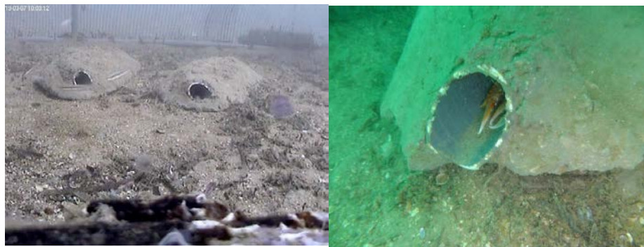
Figure 2.1.2. Images of the created enclosure in PVC material holding a contention net plus PVC tunnels embedded in concrete material, as deployed in front of the small satellite camera of the OBSEA platform. A frame depicting an animal in “door-keeping” behaviour ( sensu Aguzzi et al., 2007) is also reported.
