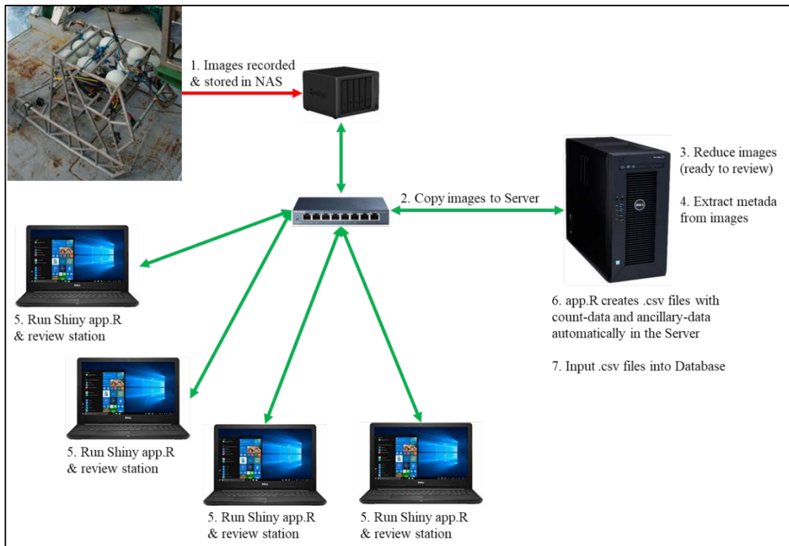
Figure 2.3.4. Diagram showing the workflow and local network of the new HD system onboard.
