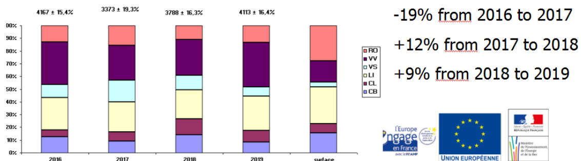
Figure 3: Time series of mean density and total abundance (with confidence intervals) with reference levels.
