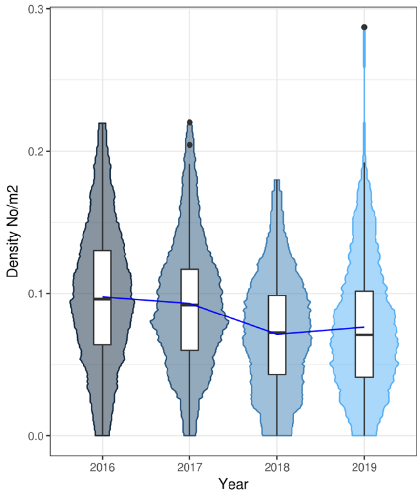
Fig 2. FU1 Iceland: Violin and box plot of adjusted burrow density distributions by year from 2016 - 2019. The blue line indicates the mean density over time. The horizontal black line represents the median, white box is the inter quartile range, the black vertical line is the range and the black dots are outliers.
