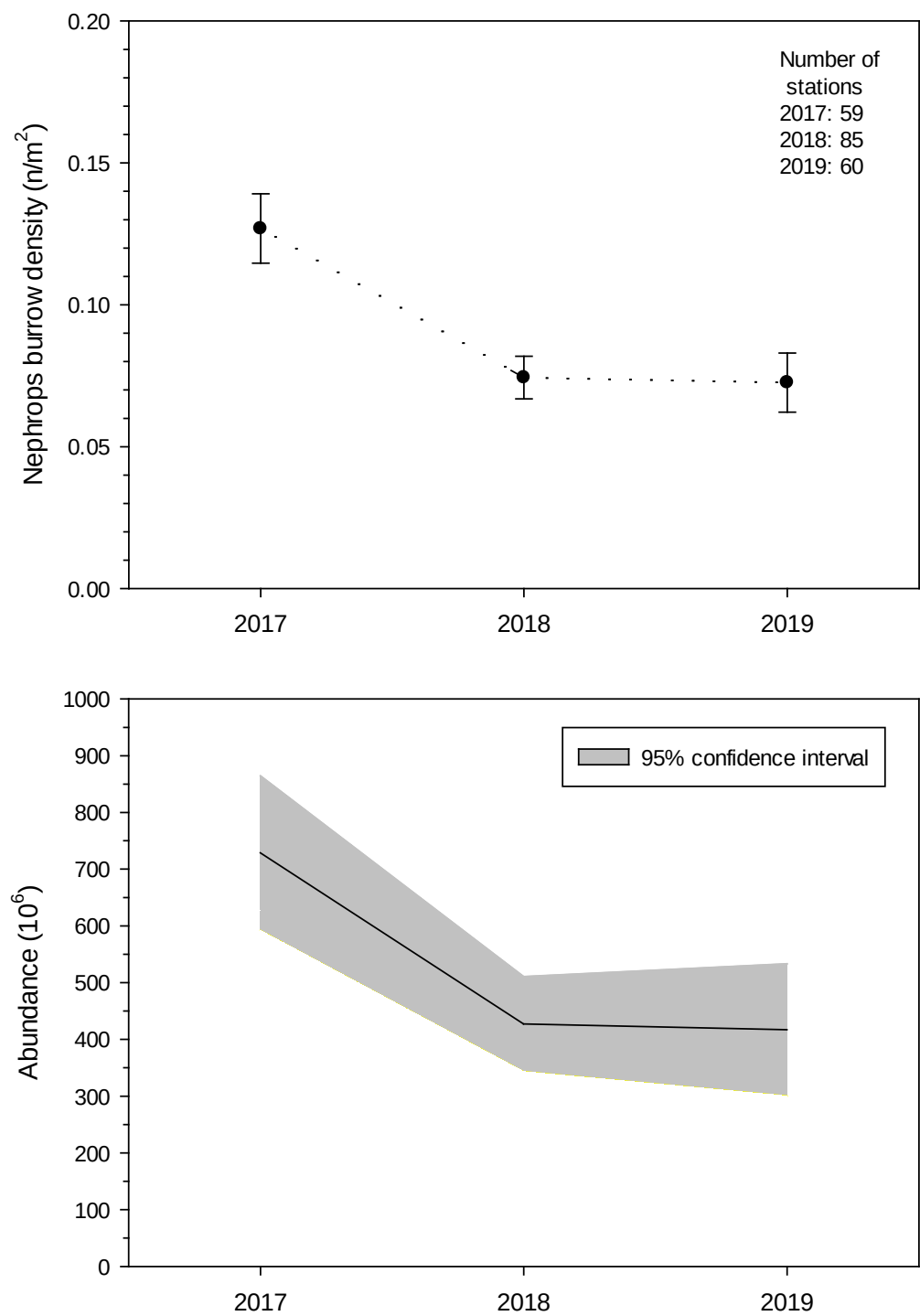
Figure 3: FU 33 (Off Horns Rev) time series of Nephrops burrow mean density and total abundance with reference levels (error bars in upper panel represent standard error of the mean and the shaded area in the lower panel represents the 95% confidence interval; reference points are not defined for this stock).
