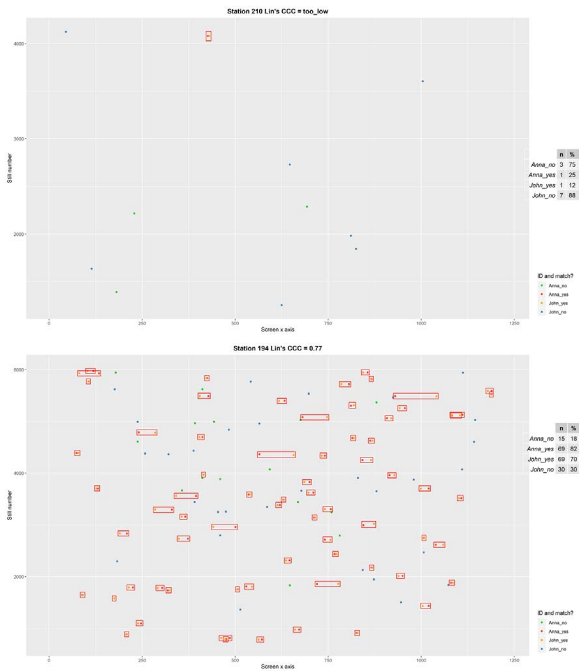
Figure 2.3.5.B. Burrow matching method. Different stations (top and bottom panel).
