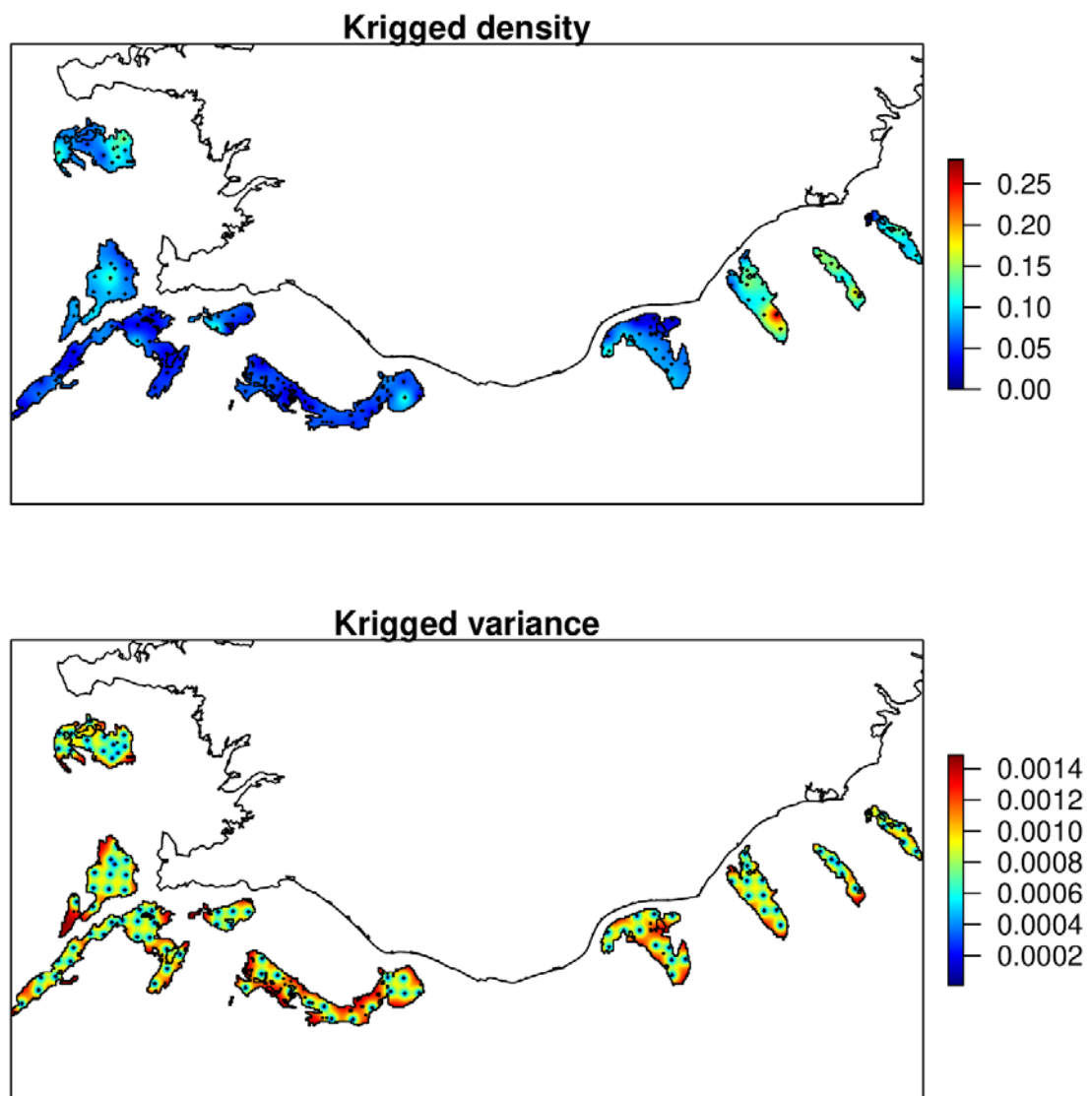
Fig 1. FU1 grounds: Contour plots of the kriged burrow density (per 100m 2 ) estimates (above) and kriged variance (below), from the 2019 survey. Black crosses represent the stations.
