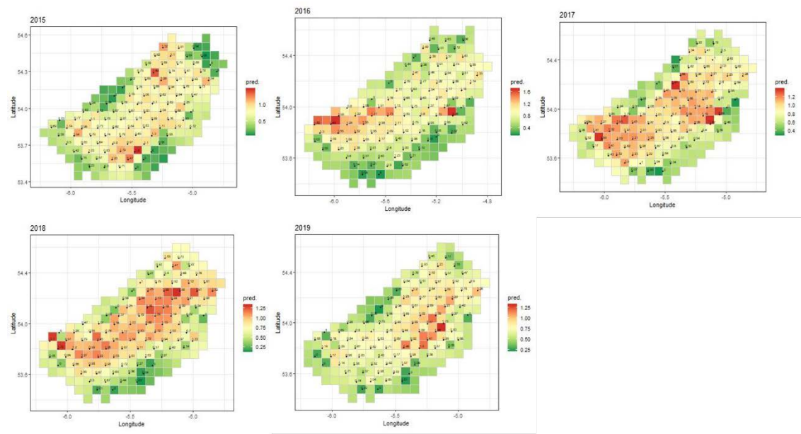
Figure 1: Map of kriged density by station for 2015 – 2019.
