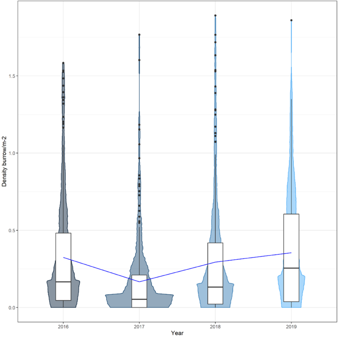
Figure 2: Times series of adjusted burrow density (Violin and box plot).
