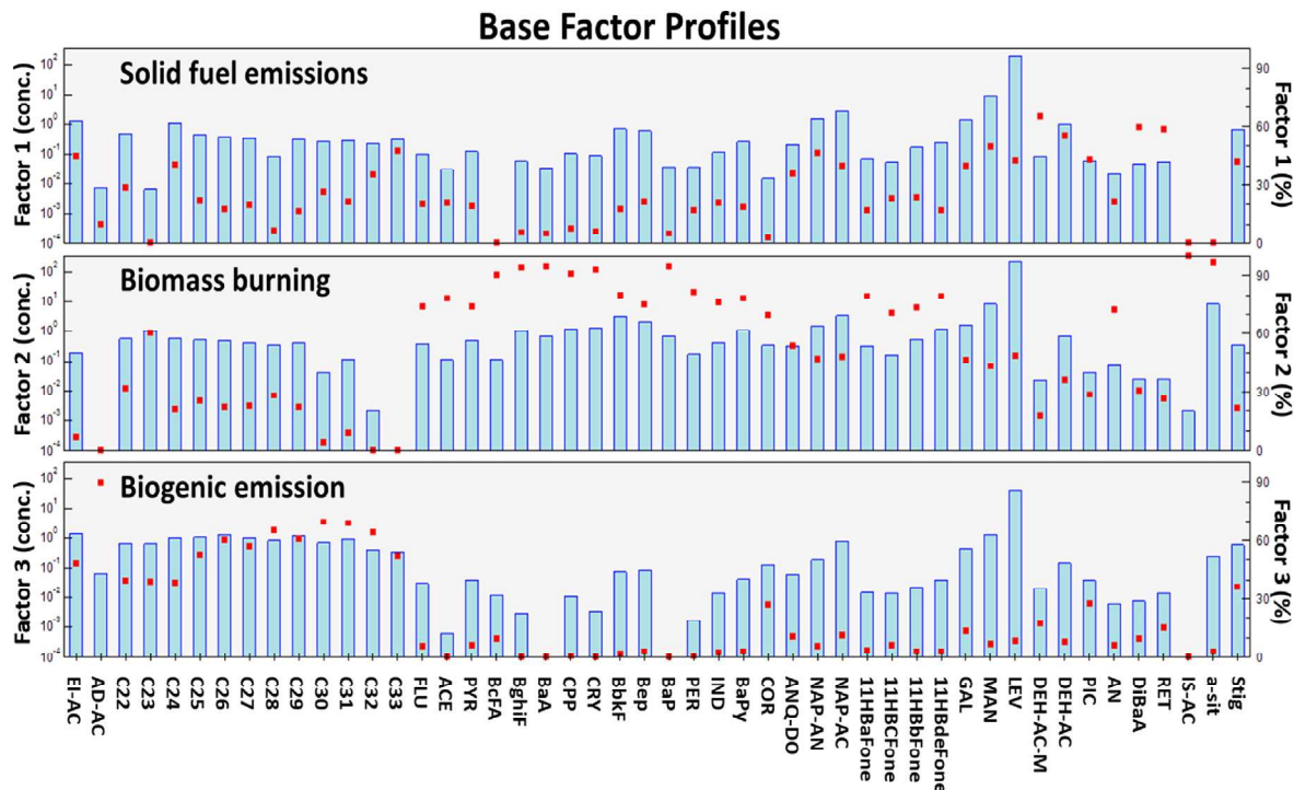
Fig. 4. PM1 and PM2.5 PMF factor profile. Solid bars correspond to concentrations and red points correspond to the percentage of species. (For interpretation of the references to colour in this figure legend, the reader is referred to the Web version of this article.)
