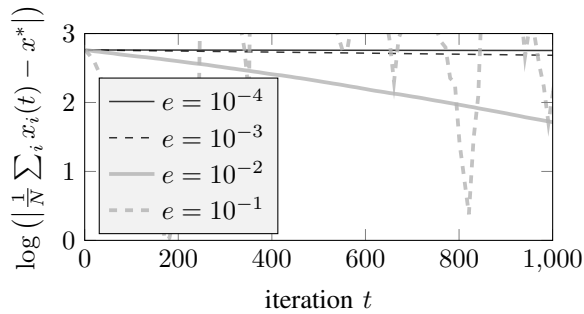
Fig. 2. Comparison of the evolutions of the trajectories of the average errors for different values of \varepsilon and a packets loss probability p = 0.1 .
