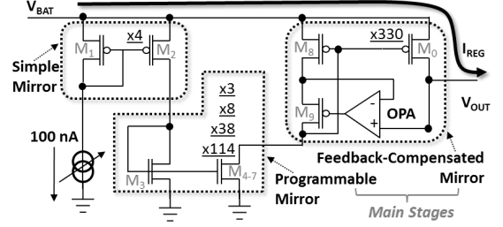
Fig. 2 Schematic of the current limiter
